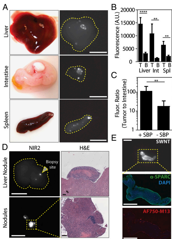
Fig. 3. Specificity of SBP-M13-SWNTs for OVCA8 tumor nodules in the abdominal cavity. (A) Photographs and NIR2 fluorescence (10–50-ms exposure) of tumor nodules implanted on several peritoneal organs. (B) Quantification of nodule and organ-specific background for nodules present on the liver, intestine, and spleen ( n = 8–11 nodules per organ; **P < 0.01 ; ****P < 0.0001 ; two-tailed t tests). (C) Tumor-to-intestine ratio for targeted and untargeted M13-SWNT probes. Intestinal tissue used for background intensity (+SBP, n = 6 ; -SBP, n = 13 ; **P < 0.01 ; two-tailed t test). (D) Representative NIR2 fluorescence and H&E staining of a positive nodule revealing characteristic tumor histology. (E) Immunofluorescence staining reveals colocalization of M13-SBP-SWNTs conjugated to AlexaFluor750 dye with SPARC expression in an NIR2-positive nodule. [Scale bars, 10 mm (A), 10 mm (D, NIR2), 250 \mu m (D, H&E liver nodule), 125 \mu m (D, H&E nodules), 5 mm (E, NIR2), and 2.5 mm (E, SPARC, AF750-M13).]
